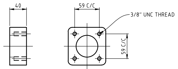
DETAIL 1 - INLET & OUTLET
